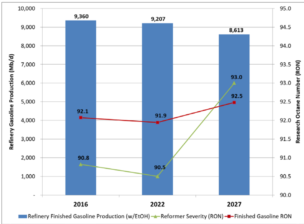
FIGURE 5 REFINERY GASOLINE PRODUCTION AND OCTANE REQUIREMENTS
